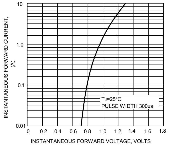
FIG.4-TYPICAL FORWARD CHARACTERISTICS
