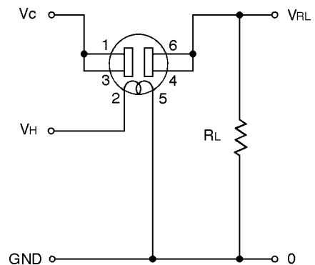
Pin #2 is indicated by a white dot on the sensor's base.
