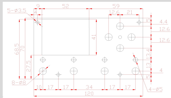
Display Board Shelf Mounting Dimensions
