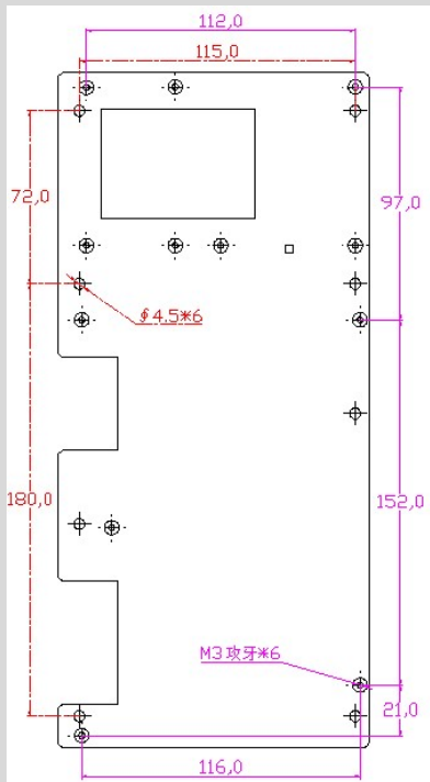
Installation Dimension
