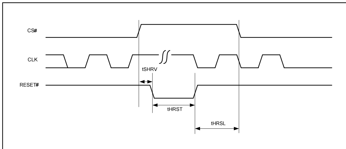
Figure 44. Reset Timing
