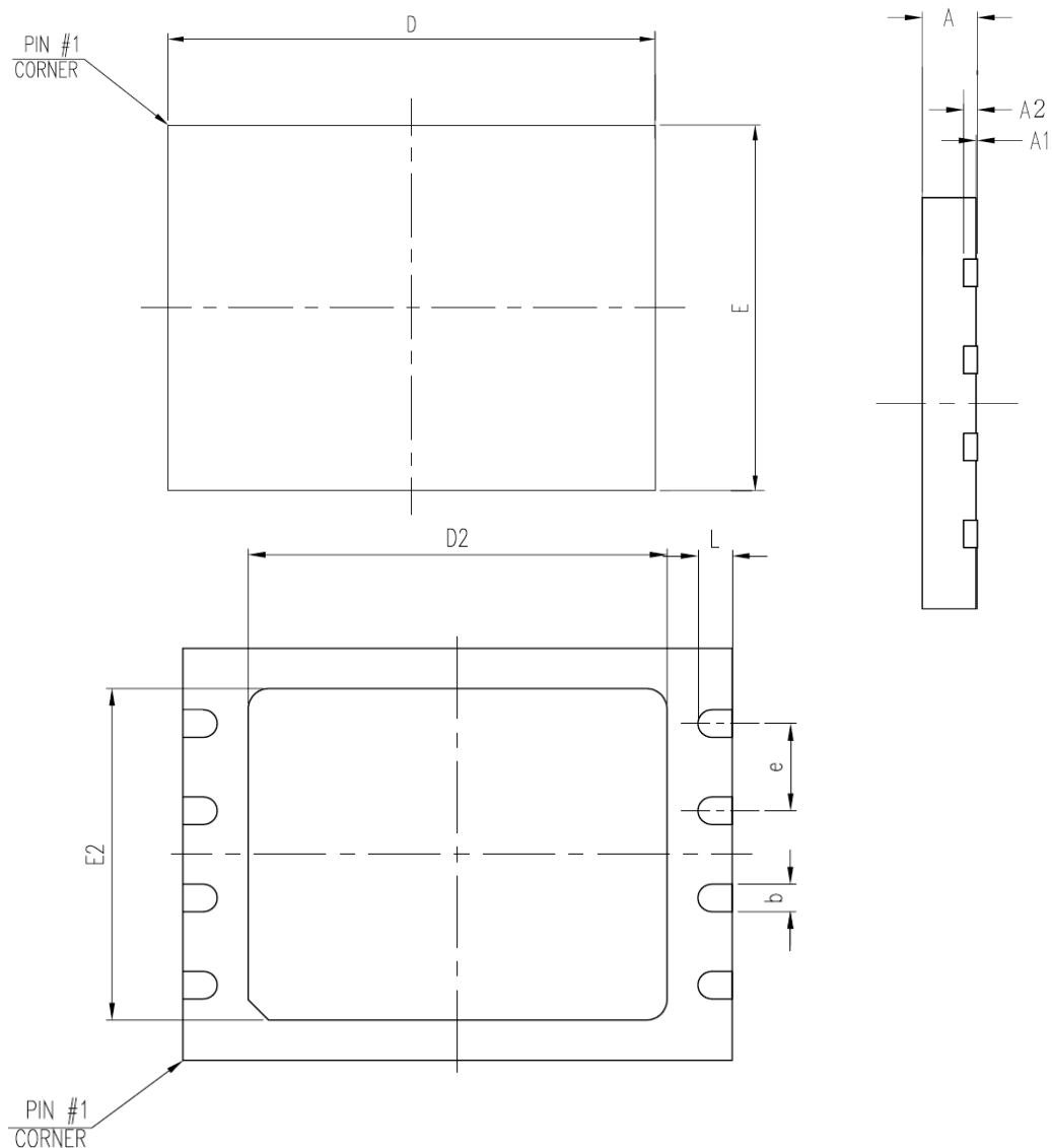
Figure 46. VDFN8 ( 5x6mm )
