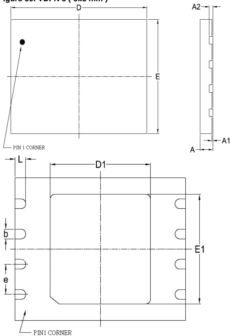
Figure 50. VDFN 8 ( 6x8 mm )
