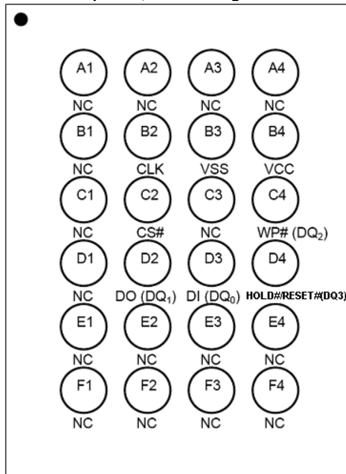
24 - Ball TFBGA
