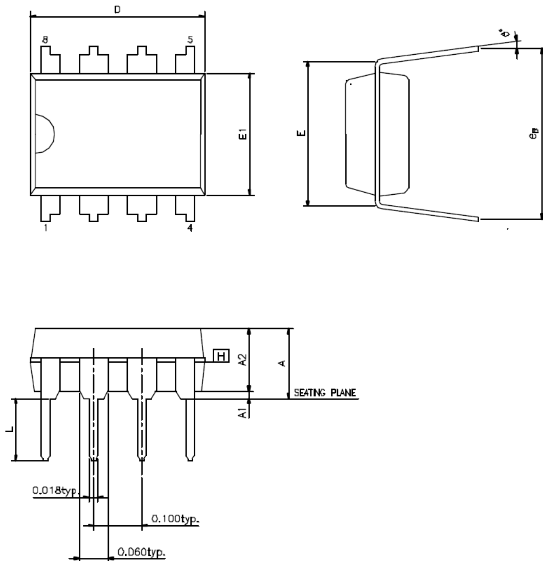
Figure 47. PDIP8
